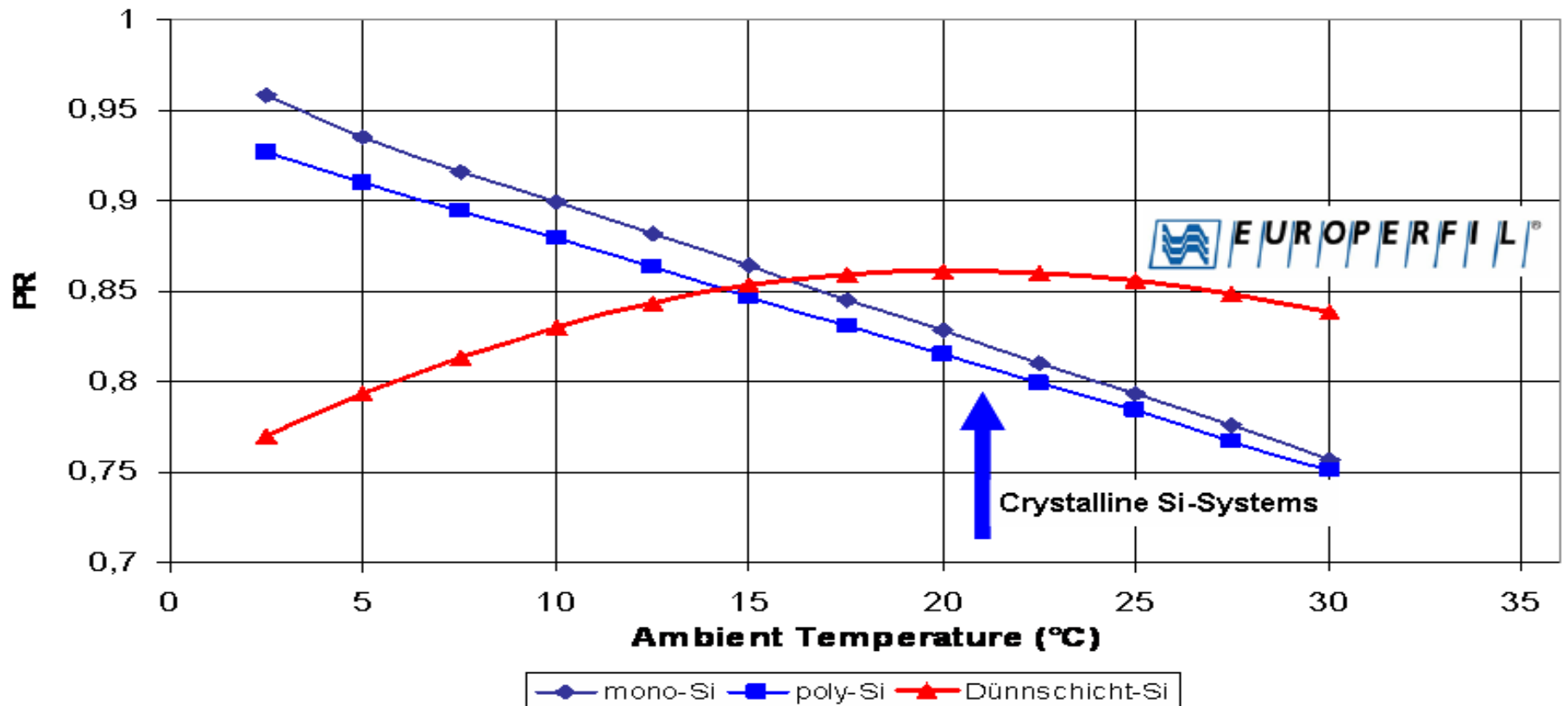
Performance Ratio (PR) of module vs. initial power (source: TISO)
